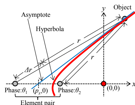
Fig. 2 Hyperbola by phase difference
