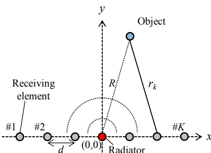
Fig. 1 Antenna configuration
