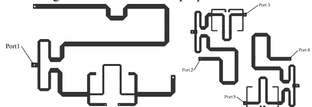
(a) Broadband 180° hybrid (b) Broadband 90° hybrid
