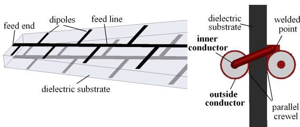
Fig. 1. Structure of the printed log-periodic antenna.
