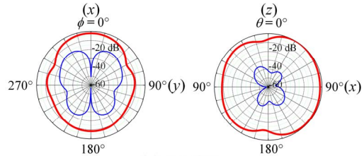
(c) 9.5 GHz
