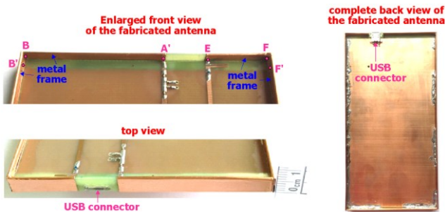
Fig. 4. Photos of the fabricated antenna.
