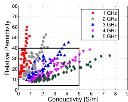
Fig. 1. Electrical parameters for 51 sample phantoms.
