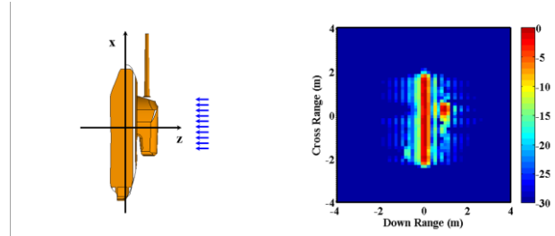
Fig. 3. Tank CAD (left) and ISAR image (right).
