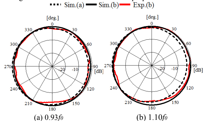
Fig. 4. Radiation pattern in horizontal plane (xy-plane).
