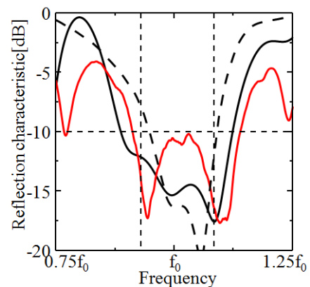
Fig. 3. Reflection characteristic of the proposed antenna.
