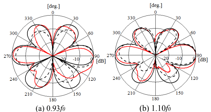
Fig. 5. Radiation pattern in vertical plane (yz-plane).
