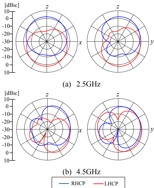
Fig. 4 Simulated radiation patterns
