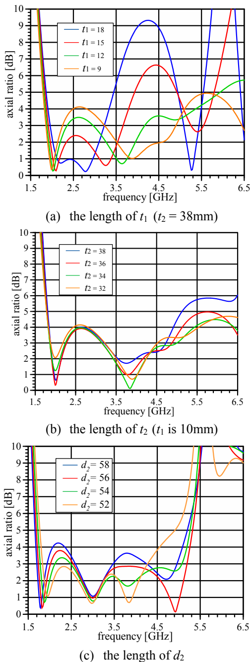
Fig. 2 Simulated axial ratio for changes of geometric parameters
