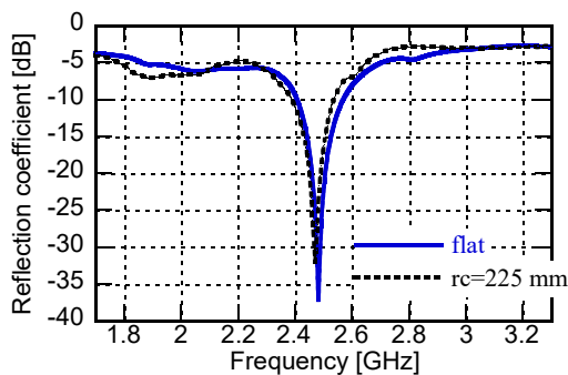
Fig. 3. Reflection characteristics.
