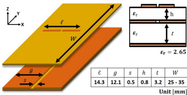
Fig. 1. Design parameters.
