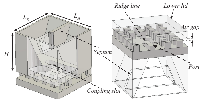
Fig. 1. The proposed horn unit cell ( L_E = 6 \text{ mm} , L_H = 6.1 \text{ mm} , and H = 5 \text{ mm} )
