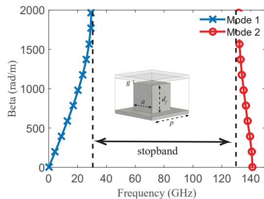
Fig. 2. Dispersion diagram of the infinite periodic pin unit cell ( d_f = 0.68 \text{ mm} , a = 0.64 \text{ mm} , g = 0.04 \text{ mm} , and p = 1.28 \text{ mm} ).
