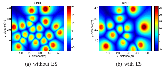
Fig. 8: SINR distribution in Reg-3 during traffic valley phase
