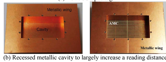
Fig. 4. Long-range single- or dual-band tag antennas installed in metallic cavities with or without an AMC ground plane [5, 6].
