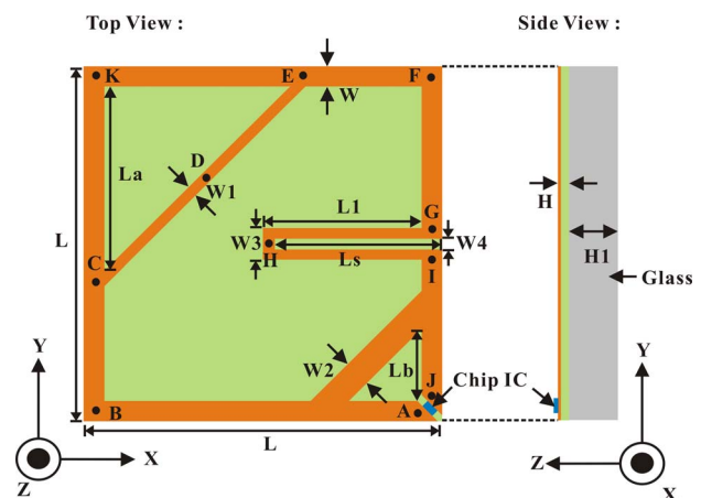
Fig. 1. Geometry of the proposed compact circularly polarized (CP) tag antenna for UHF RFID system.
