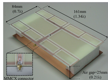
Fig. 2. Photograph of the fabricated 2 \times 2 array antenna with the reflector.
