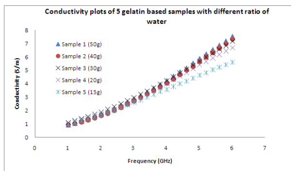
Fig. 2. Conductivity of 5 gelatin based samples with different ratio of water.
