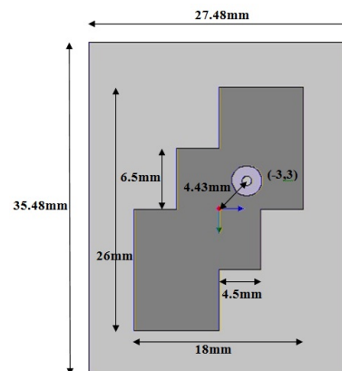
Fig. 1. Antenna geometry with feed location.
