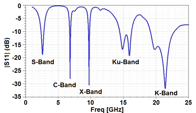
Fig. 2. Predicted |S_{11}| when feed is located at (-3, 3).
