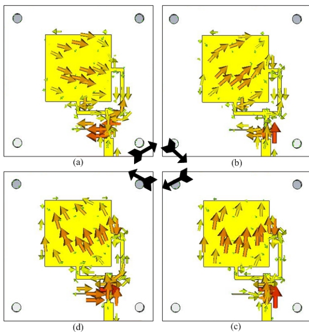
Fig. 2. Vector current distribution of designed RMA for various source phase: (a) \varphi_s = 0^\circ ; (b) \varphi_s = 45^\circ ; (c) \varphi_s = 90^\circ , and (d) \varphi_s = 135^\circ
