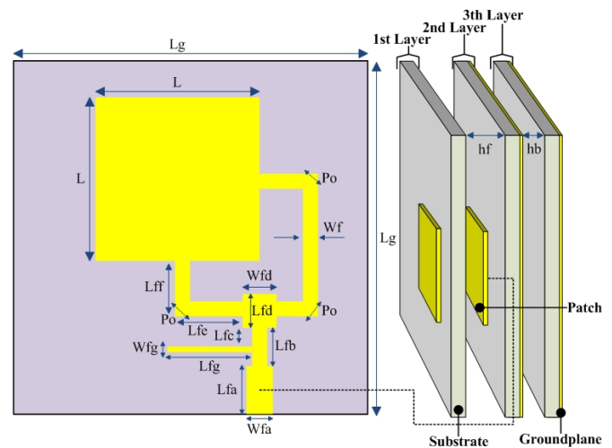
Fig. 1. Geometry of Dual-fed orthogonal RMA second layer top view, and side view.
