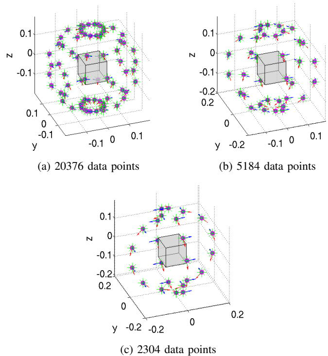
Fig. 3. Three dipole configurations with antenna positions (dots) on a sphere with radius 0.2m . The arrows in two orthogonal directions indicate transmitting dipoles. The cube in the center indicates the reconstruction domain \mathcal{D} .
