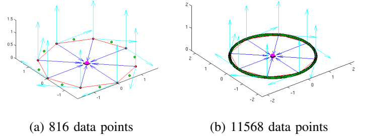
Fig. 2. Two dipole configurations with antenna positions (dots) on a circle with radius 1.67m. The arrows in two orthogonal directions indicate transmitting dipoles. The highlighted region in the center indicates the reconstruction domain \mathcal{D} .
