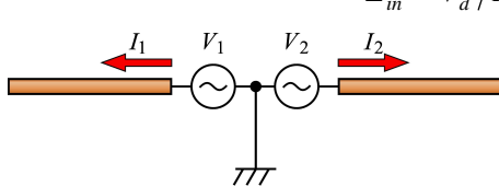
Figure 1: Dipole antenna.
