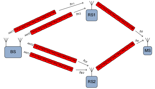
Fig. 2. Simple cooperative relaying with virtual OSTBC
