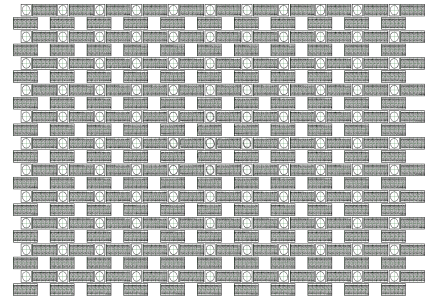
Figure 6: Observation phase-waves in domain D ( \alpha=0.05 , \varepsilon=0.47 ).
