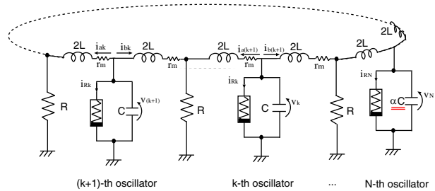
(a) Ring of van der Pol oscillators.
