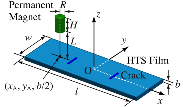
Figure 1: A schematic view of a scanning permanent magnet method.
