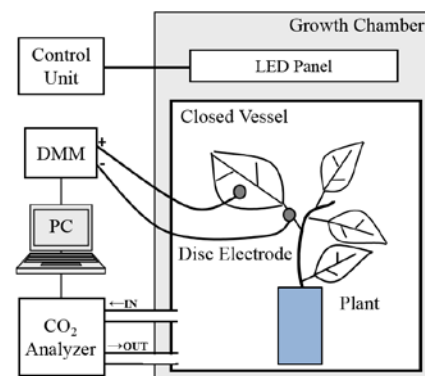
Figure 1. Previous measurement system.
