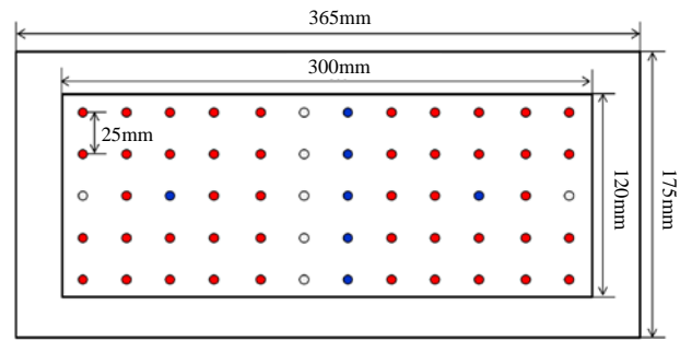
Figure 5. Pattern arrangement of LEDs light source. ( ● : blue, ● : red, ○ : white)
