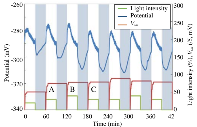
Figure 7. Example of automatic light intensity control
