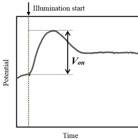
Figure 2. Typical bioelectric potential response to light irradiation and definition of evaluation parameter, V_{on} .
