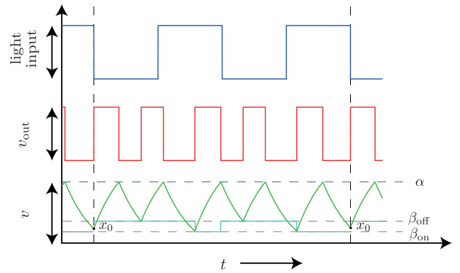
Figure 3: Isolated periodic waveform , \alpha_{\text{off}} = \alpha_{\text{on}} = 0.7577 , \beta_{\text{off}} = 0.5155 , \beta_{\text{on}} = 0.0021 , T = 4.0 .
