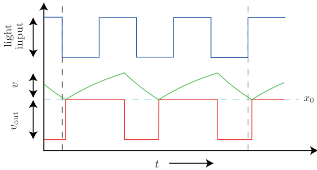
Figure 4: Border-Collision bifurcation , \beta_{\text{off}} = x_0 .
