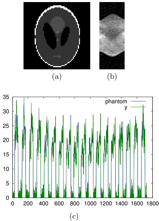
Figure 2: (a) phantom, (b) sinogram, and (c) projections with and without noise
