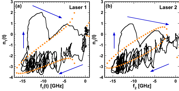
Figure 4: Trajectories of the low-frequency fluctuations of the mutually coupled lasers in the phase space for (a) laser 1 and (b) laser 2. The phase space consists of the optical frequency and the carrier density. The orange circles indicate the steady state solutions. The blue arrows represent the direction of change in the trajectories.
