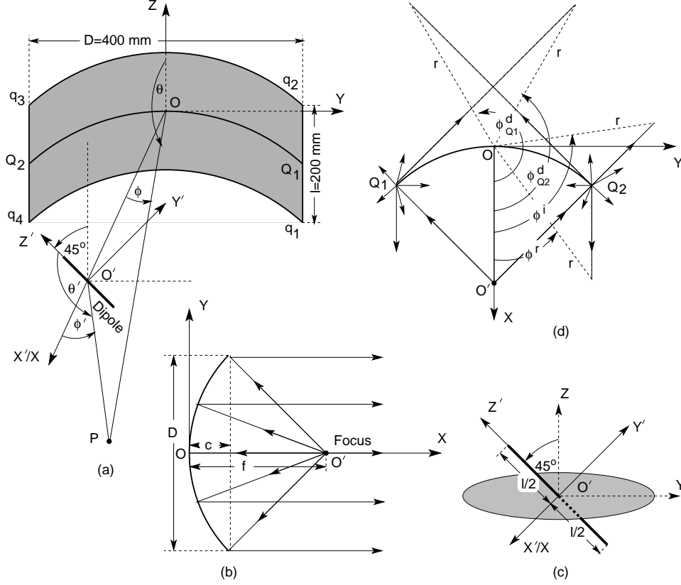
Figure 1: (a) Geometry for parabolic cylindrical reflector. Feed dipole antenna set at a slant of 45°. (b) Dimensions. (c) Dipole at a slant of 45°. (d) Diffraction from edges of the reflector and boundary angles.
