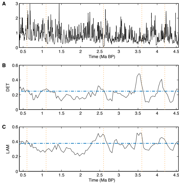
Figure 3: (A) Dust flux record of ODP site 659, and corresponding (B) DET and (C) LAM measures (95% confidence bounds are shown with blue dash-dotted lines).
