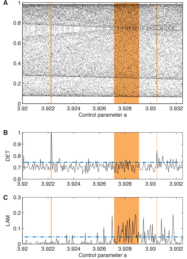
Figure 1: (A) Logistic map with chaos-period and chaos-chaos transitions for control parameter a = [3.9200 \ 3.9325] and corresponding RQA measures (B) DET and (C) LAM . For a = [3.92221 \ 3.92227] we have a period-7 window, for a = [3.93047 \ 3.93050] a period-8 window and at a broad range around a = 3.928 intermittency (highlighted with orange bars). 99% confidence bounds are shown as blue dash-dotted lines.
