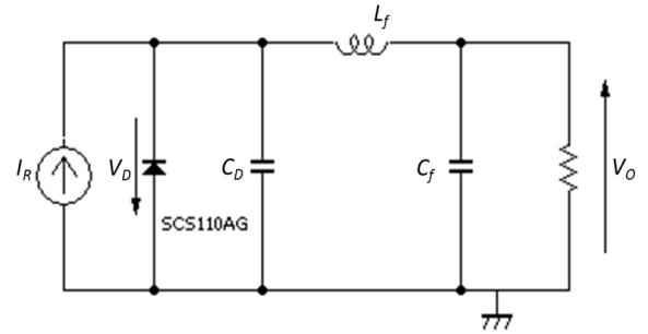
Figure 4: Configuration of class E rectifier.
