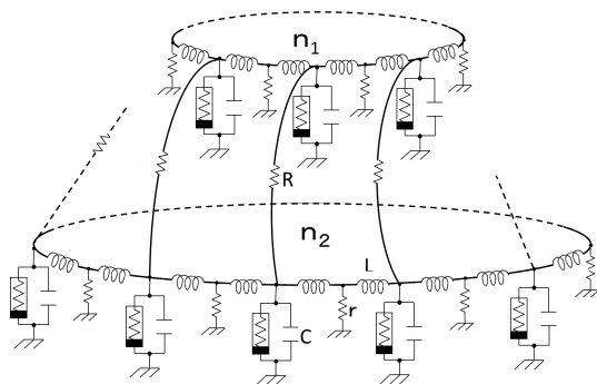
Figure 1: Two rings of coupled oscillators.
