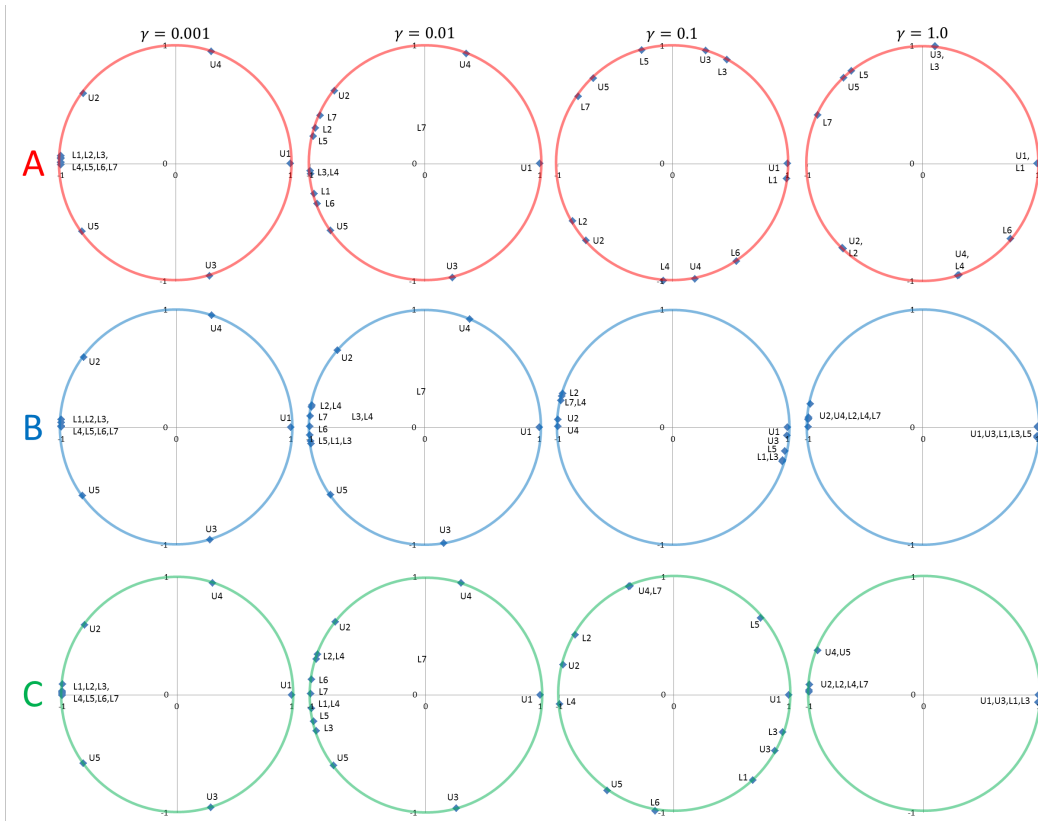
Figure 9: Average phase for different \gamma .
