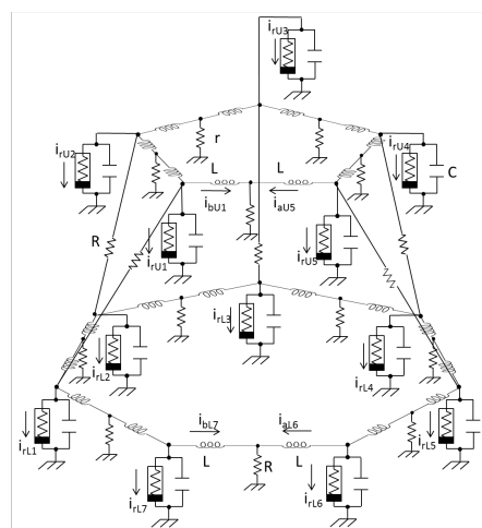
Figure 3: Circuit model of 5-7 rings.
