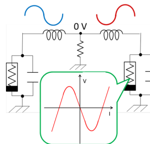
Figure 2: Anti-phase of two oscillators.
