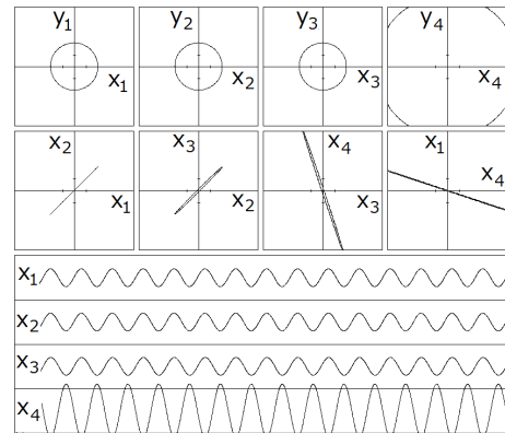
Figure 7: Computer simulation results when n = 4 , \beta_4 = 3 .
