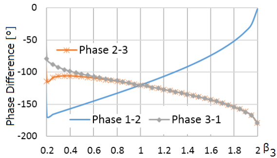
Figure 5: Computer simulation results when n = 3 .
