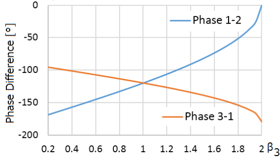
Figure 3: Theoretical analysis results when n = 3 .
