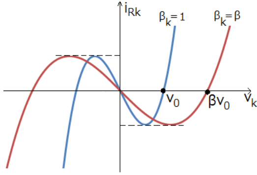
Figure 2: Relation between amplitude and \beta_k .
