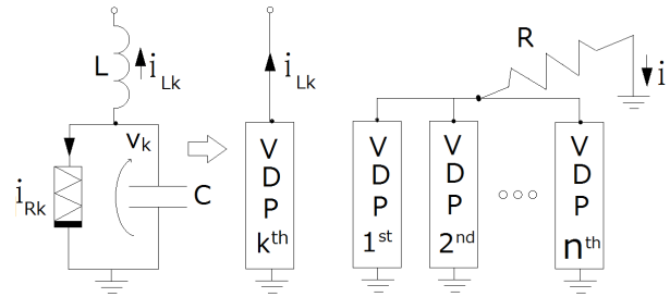
Figure 1: Circuit model.
