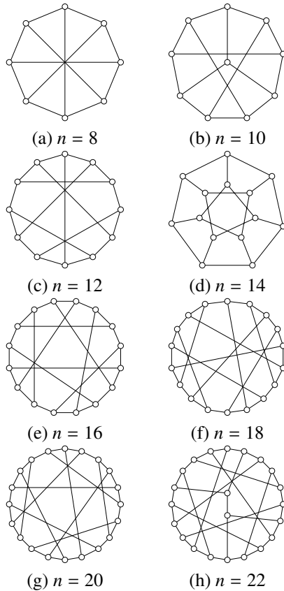
Figure 2: ACLM graphs obtained by Algorithm 1.
