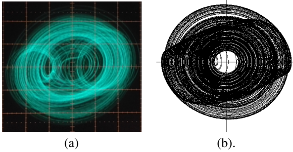
Figure 3: Circuit experimental result and computer simulation result of a MBCC. (a) Horizontal axis is i_{k1} . Vertical axis is v_{k2} . R_{k1} = 1800 [ \Omega ], C_{k1} = 6.8 [nF], C_{k2} = 68 [ \mu F], L_{k1} = 20 [mF], R_m = 10 [k \Omega ], C_m = 10 [nF], R_r = 1000 [k \Omega ], R_1 = 2 [k \Omega ], R_2 = 2 [k \Omega ], R_3 = 1.48 [ \Omega ], R_4 = 30 [k \Omega ] and R_5 = 30 [k \Omega ]. (b) Horizontal axis is x_{k4} . Vertical axis is x_{k3} . \alpha = 0.037 , \beta_a = 11 , \beta_b = 10 , \gamma_a = 0.28 , \gamma_b = 0.29 , M_1 = -0.379 , M_2 = 0.065 , \delta = 0.09 , \varepsilon = 1.1 and \zeta = 1.0 .
