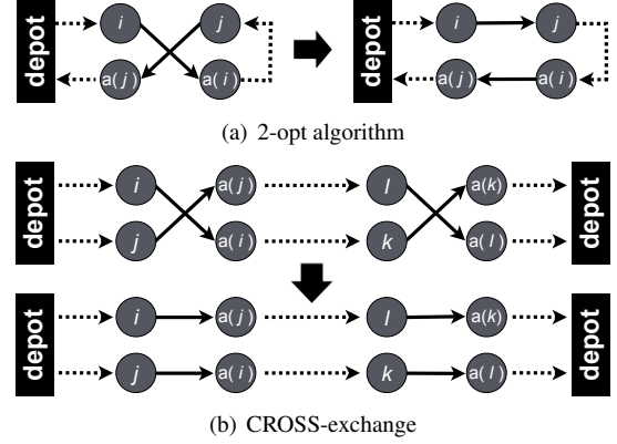
Figure 1: Graphical representation of local search methods. In this example, a(i) is the next city to i . In (a), two paths ( i-a(i) and j-a(j) ) are deleted from the current tour, then new two paths, i-j and a(j)-a(i) , are added. In (b), a partial tour a(i) \cdots k in one tour and a partial tour a(j) \cdots l in the others are exchanged.
