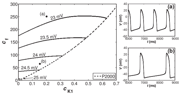
Figure 9: Contour curves of overshoot.
