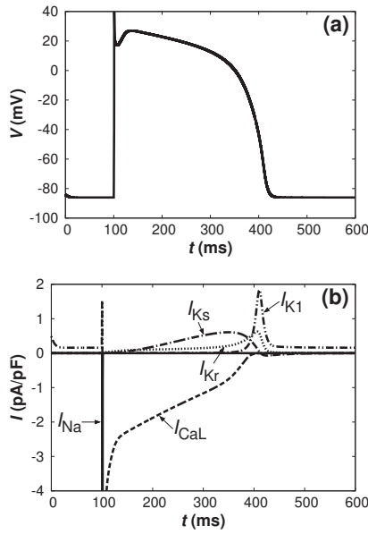
Figure 1: Action potential simulated by the reduced TNNP model, (a) membrane potential, (b) ionic current (negative current denotes inward current).
