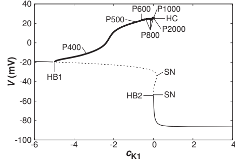
Figure 2: One-parameter bifurcation diagram as to c_{K1} . Solid and broken curves denote stable and unstable solution, respectively. Thick and thin curves denote the maximum value of periodic solution and equilibrium points, respectively.
