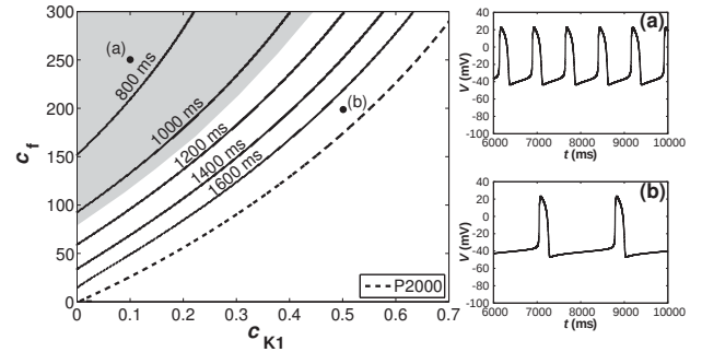
Figure 7: Contour curves of period.
