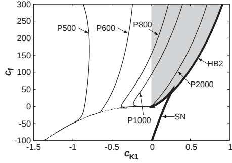
Figure 4: Two-parameter bifurcation diagram as to the two bifurcation parameters c_{K1} and c_f . Solid and broken curves denote stable and unstable solution, respectively.
