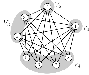
Figure 2: Complete 4-partite graph K_{1,1,2,4} . The algebraic connectivity of this graph is 4.
