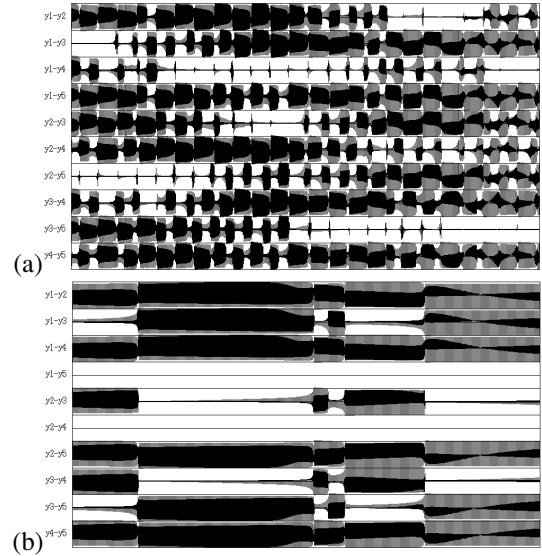
Figure 12: Synchronization of five chaos. \varepsilon = 0.75 , \alpha = 0.80 and \omega = 1.10 . (a) \gamma = 0.17 . (a) \gamma = 0.50 .
