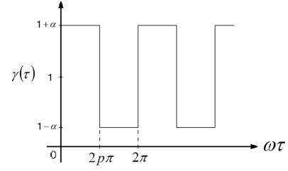
Figure 5: Function relating to parametrically excitation.
