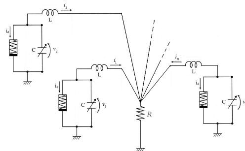
Figure 1: Circuit model.
