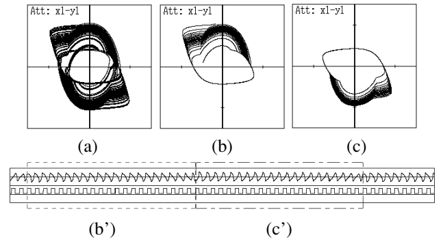
Figure 6: Attractors, time series and rectangular wave relating to parametrically excitation \varepsilon = 0.75 , \alpha = 0.80 and \omega = 1.10 .
