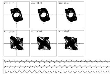
Figure 9: Self-switching phenomena of in-phase synchronization and opposite-phase synchronization. \varepsilon = 0.75 , \alpha = 0.80 , \omega = 1.10 and \gamma = 0.10 .
