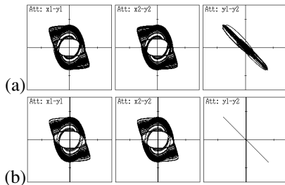
Figure 8: Synchronization of two chaos. \varepsilon = 0.75 , \alpha = 0.80 and \omega = 1.10 . (a) \gamma = 0.001 . (b) \gamma = 0.01 .
