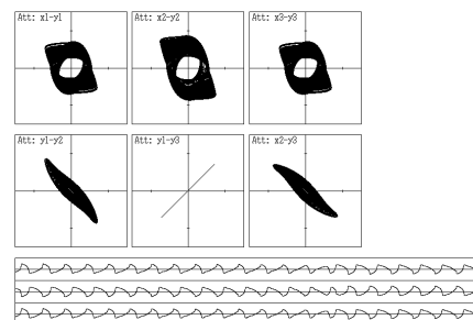
Figure 10: Synchronization of three chaos when initial values of two subcircuits are set as same values. \varepsilon = 0.75 , \alpha = 0.80 , \omega = 1.10 and \gamma = 0.10 .
