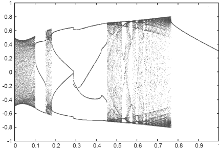
Figure 3: One-parameter bifurcation diagram for \alpha = 0.8 , \omega = 1.1 and varying \varepsilon .
