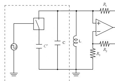
Figure 2: Subcircuit corresponds to van der Pol oscillator involving periodically forced capacitor.
