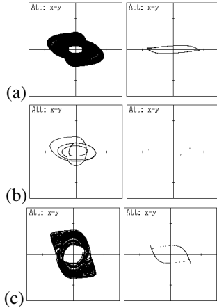
Figure 4: Attractors and Poincaré maps. \alpha = 0.8 and \omega = 1.1 . (a) \varepsilon = 0.10 . (b) \varepsilon = 0.12 . (c) \varepsilon = 0.75 .
