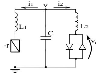
Figure 1: The model of the chaotic circuit.
