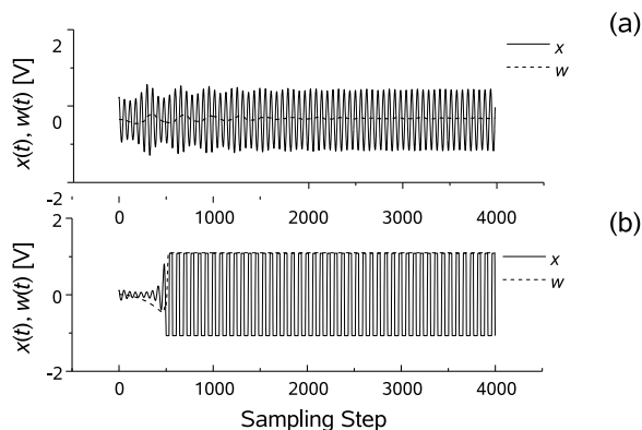
Figure 3: Linear coupling : Time series of the system variable x(t) (line) and the control loop variable w(t) (dashed) for fixed parameters \varepsilon = -0.1 , k = 0.3 and \lambda_c = 0.051 , but different initial conditions. (a) Initial conditions close to the UPO (x_0, y_0, w_0) = (0.6, 0, 0) : control successful. (b) Initial conditions close to the origin (x_0, y_0, w_0) = (0.1, 0, 0) : control fails.
