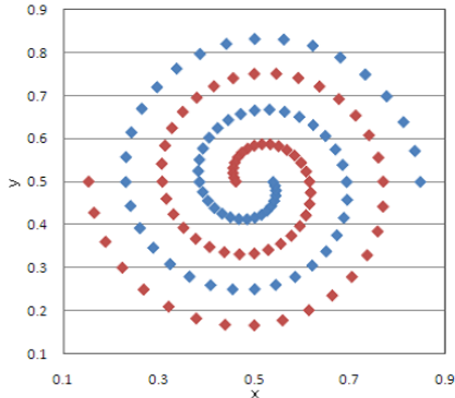
Figure 6: Two-spiral problem.
