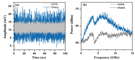
Fig. 4. The time series (a) and power spectrum (b) of the chaotic laser with (blue) and without (gray) optical feedback from each branch.
