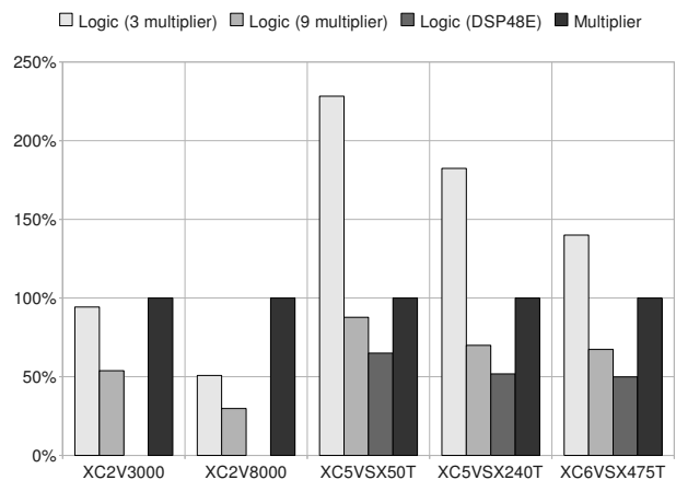
Figure 2: The logic usage in Falcon
