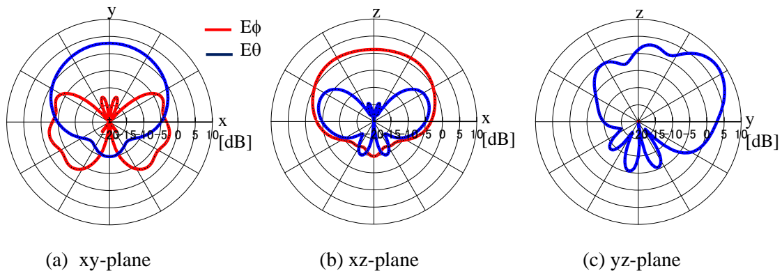
(a) xy-plane (b) xz-plane (c) yz-plane Figure 6: Calculated electric field radiation patterns of the proposed antenna at 2.45 GHz. pyp=200\text{mm} , pym=0\text{mm} , h=4.0\text{mm} , pxp1=pxm1=20.0\text{mm} , pzp1-pzp2=10.0\text{mm} , pzp2=37.0\text{mm} , pxp2=pxm2=100\text{mm} , L=30.36\text{mm} , L1=23.45\text{mm} .
