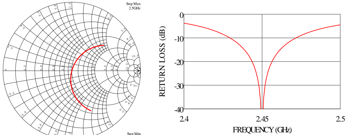
Figure 5: Calculated input impedance and return loss characteristics of proposed antenna. pyp=200\text{mm} , pym=0\text{mm} , h=4.0\text{mm} , pxp1=pxm1=20.0\text{mm} , pzp1-pzp2=10.0\text{mm} , pzp2=37.0\text{mm} , pxp2=pxm2=100\text{mm} , L=30.36\text{mm} , L1=23.45\text{mm} .
