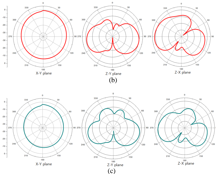
Fig. 6 Measured radiation patterns at (a) 849MHz, (b) 1920MHz, and (c) 2110MHz
