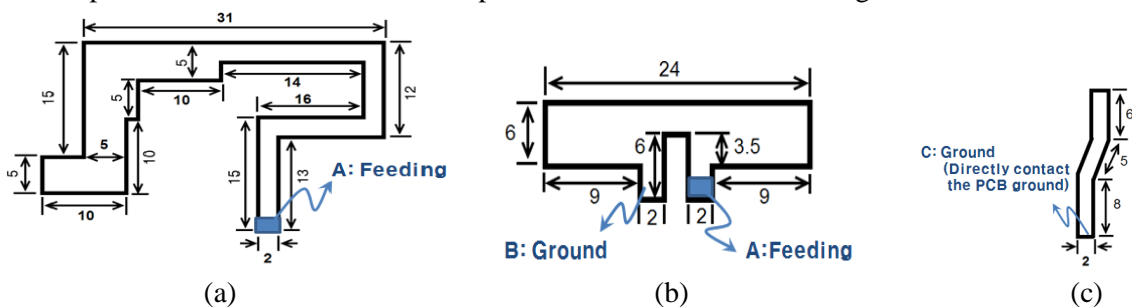
Fig. 1. The structures of the proposed multiband combo antenna: (a) Folded monopole antenna, (b) Printed loop antenna, and (c) Parasitic element.
