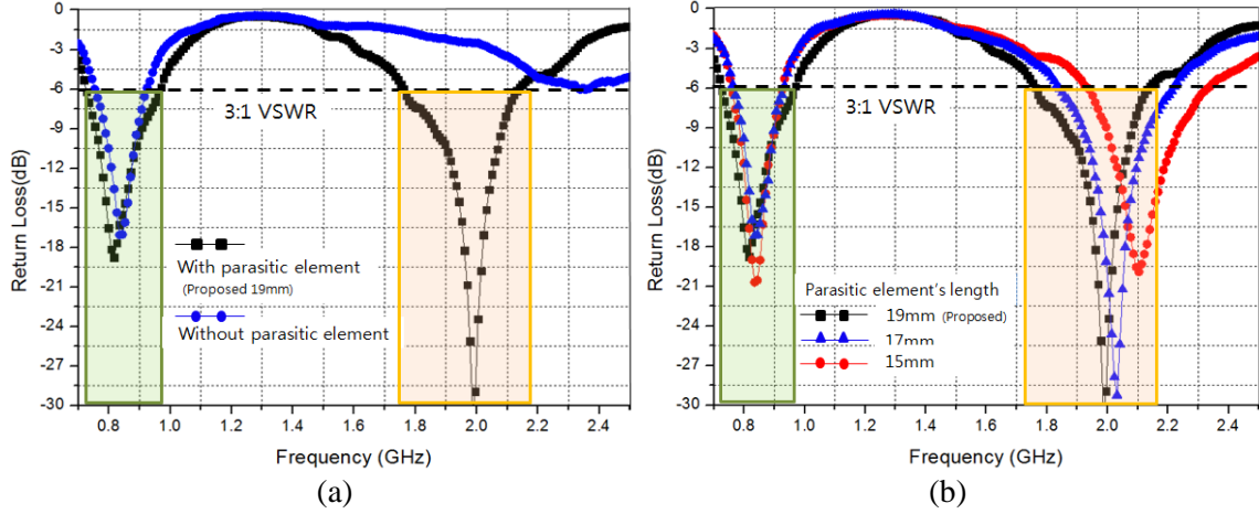
Fig.4. Comparison of the measured return losses: (a) the proposed antenna with a parasitic element (folded monopole, printed loop, and parasitic element) vs. the antenna without parasitic element (only folded monopole and printed loop), (b) Return losses according to the length of the parasitic element
