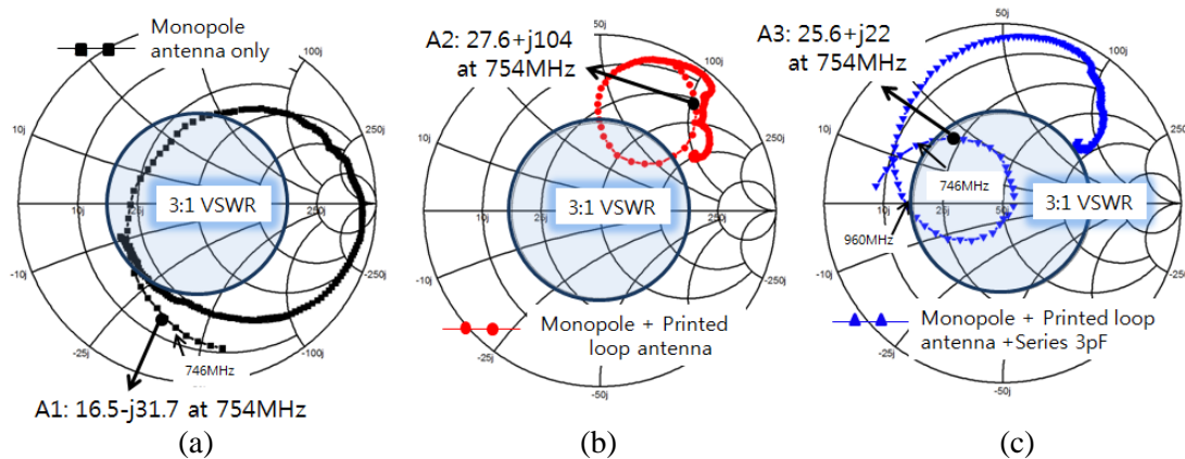
Fig. 3. Measured input impedances on the Smith chart: (a) monopole antenna only, (b) monopole antenna and printed loop antenna, and (c) monopole antenna, printed loop antenna, and a series capacitor of 3pF
