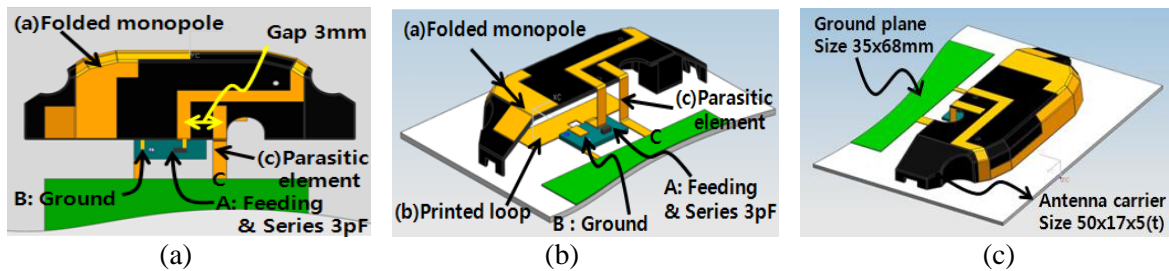
Fig. 2. Geometry of the proposed multiband combo antenna: (a) Top view, (b) and (c) 3D view
