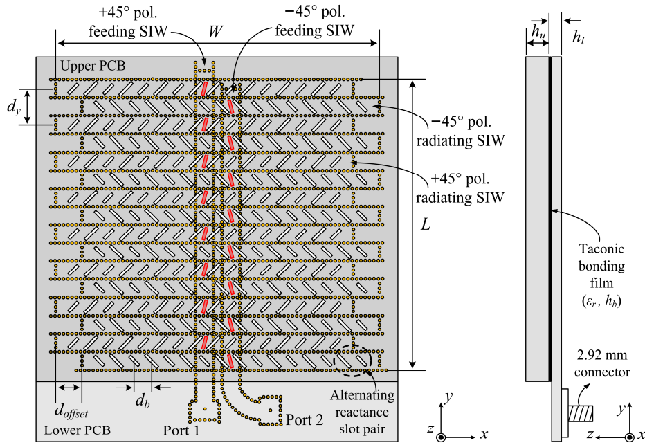
Figure 1: The perspective and lateral view of the proposed antenna.
