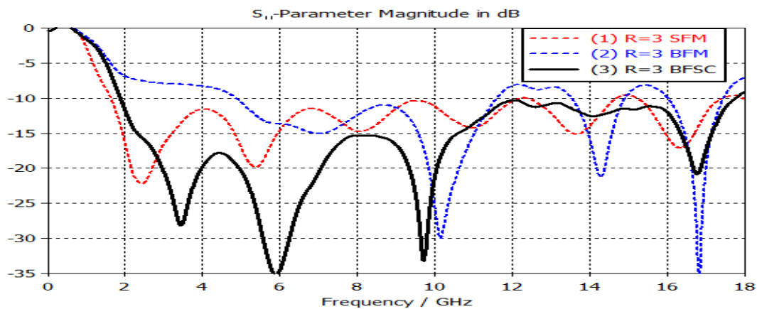
Figure. 2 Return loss curves for the three designed antennas. SFM: Straight Feed Monopole; BFM: Bended Feed Monopole; BFSC: Bended Feed Self-Complementary.
