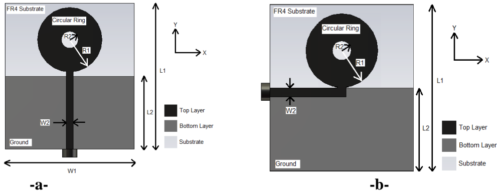
Figure 1. Geometry of the circular ring monopole antennas;- a- Antenna-1 with straight feed line, b- Antenna-2 with bended feed line.
