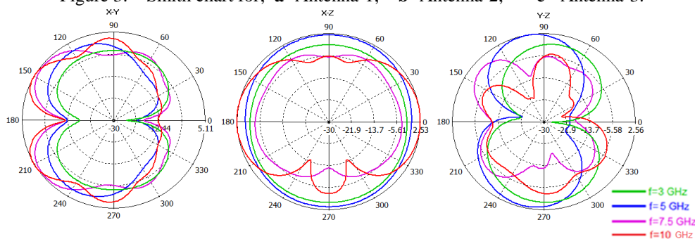
Figure 4. Radiation pattern in the three principal planes for Antenna-1.
