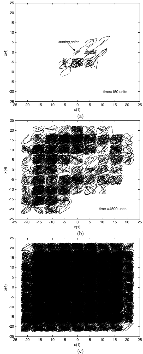
Figure 4. Hyperchaotic 9x9-scroll attractor on (x_1, x_4) -plane. (a): time t=150 ; (b): time t=4500 ; (c): final attractor.
